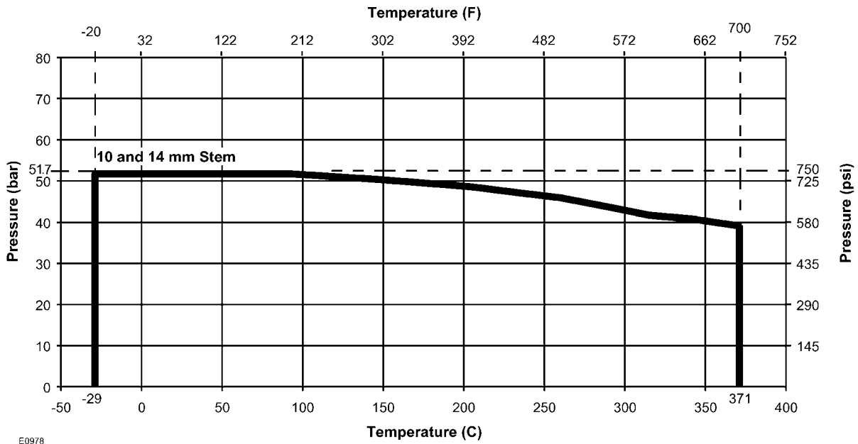
Figure 12. Bellows Pressure - Temperature Ratings
